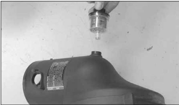
9. Remove the air filter restriction gauge and stock grommet from the air filter housing as shown.
