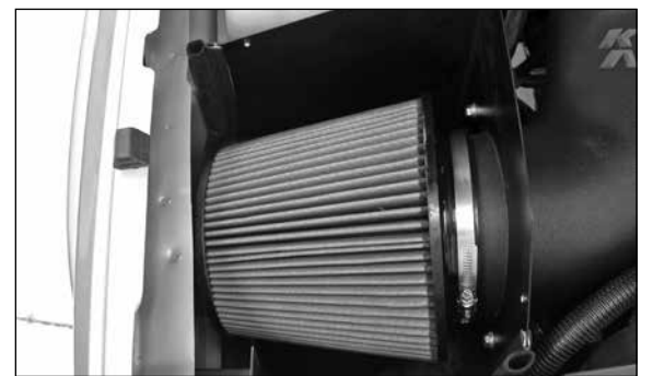
20. Install the K&N® air filter onto the K&N® intake tube and secure with the provided hose clamp.
