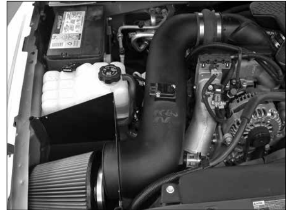
19. Secure the K&N® intake tube to the silicone hose at the throttle body with the hose clamp provided and to the heat shield with the provided hardware.
