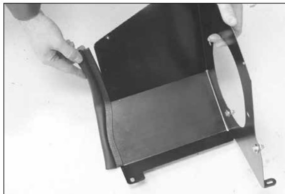
15. Install the edge trim onto the heat shield as shown. NOTE: Some trimming of the edge trim will be necessary.
