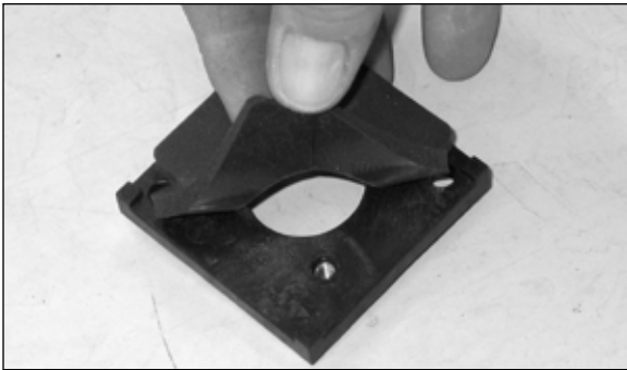
10. Attach the provided gasket onto the back of the K&N® mass air adapter as shown.
