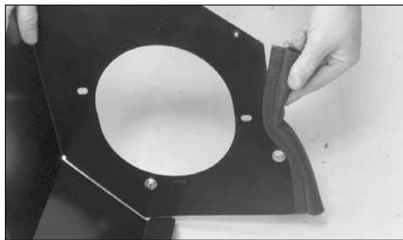
16. Install the edge trim onto the heat shield as shown. NOTE: Some trimming of the edge trim will be necessary.
