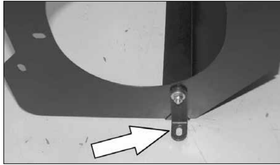
13. Install the "L" bracket (07805) onto the heat shield as shown with the provided hardware as shown.
