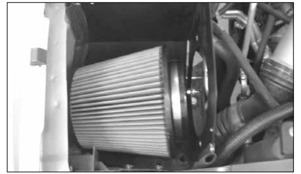
18. Set the K&N® air filter into the heat shield as shown.
